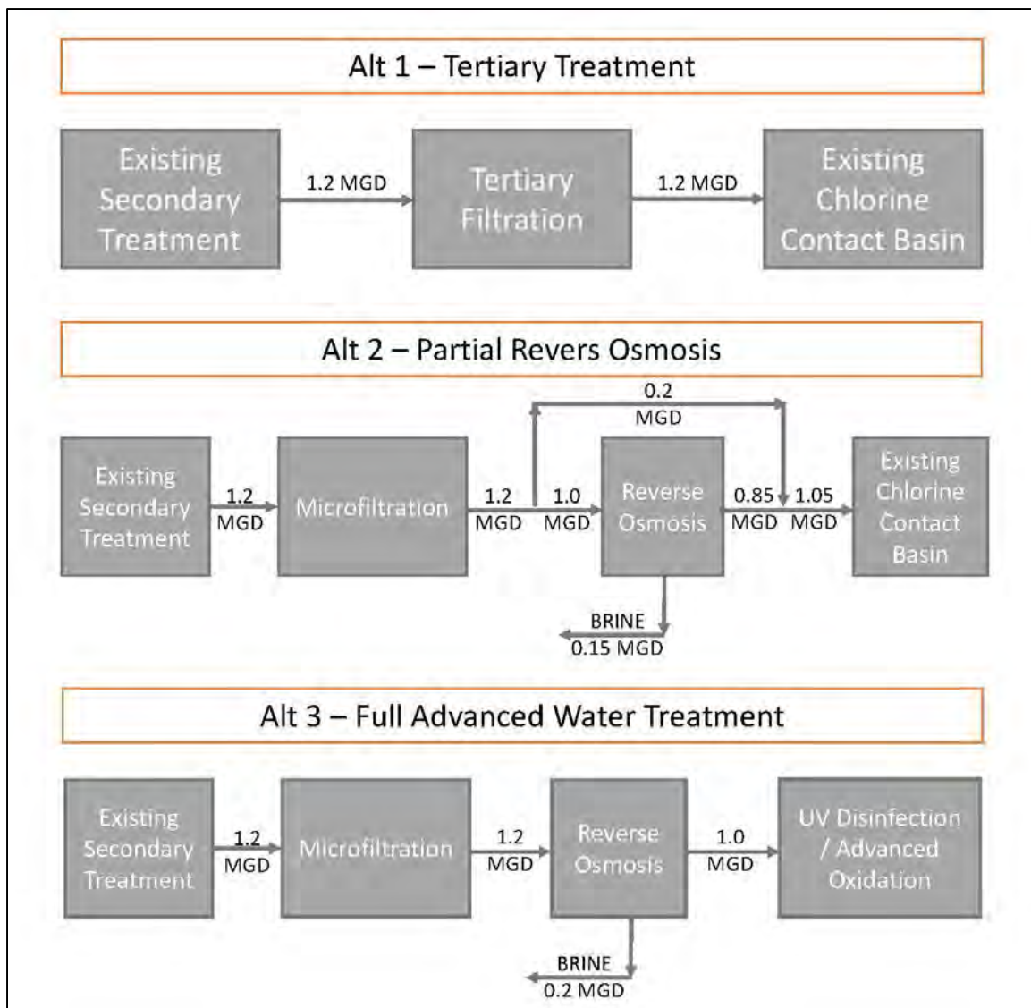
Figure 5-5: Treatment Alternatives Schematics
